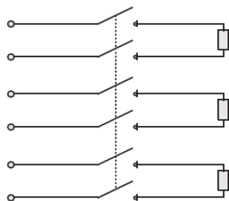
两层串联 6 层外形 Cabling across six layers
