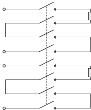
四层串联 8 层外形 Cabling across eight layers
