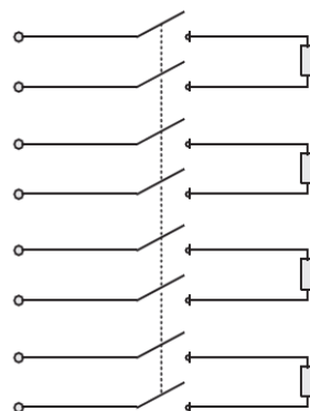
两层串联 8 层外形 Cabling across eight layers
