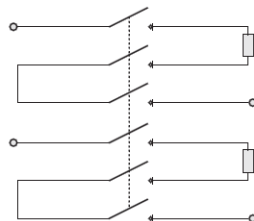
三层串联 6 层外形 Cabling across six layers
