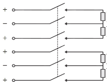
两正共负 6 层外形 Cabling across six layers
