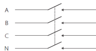
交流 4 层产品接线图 Cabling across four layers
